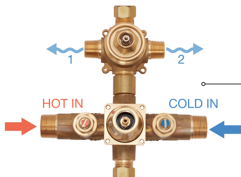
1/2" Thermostatic Shower Valve Model #18.30.910 $495
