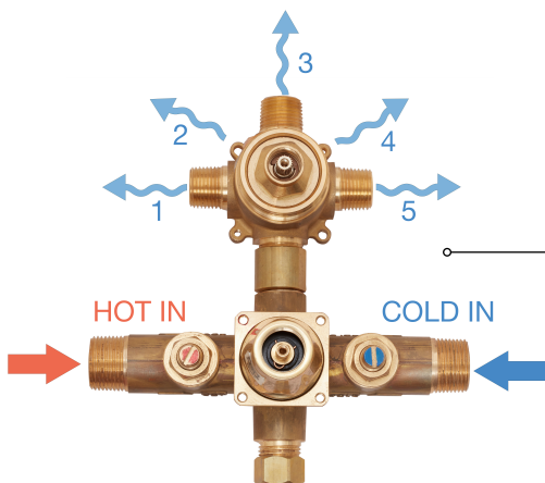
1/2" Thermostatic Shower Valve Model #18.30.912 $525
